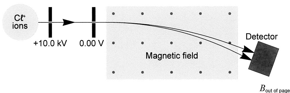
Schematic of a mass spectrometer
